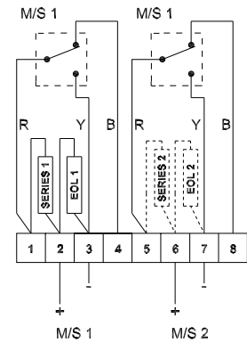
8A - Circuit shown in Unoperated condition (Glass Intact) Terminals +(2) & -(3) M/S 1 and +(6) & -(7) M/S 2 open Terminals +(2) & (4) M/S 1 and +(6) & (8) M/S 2 closed
