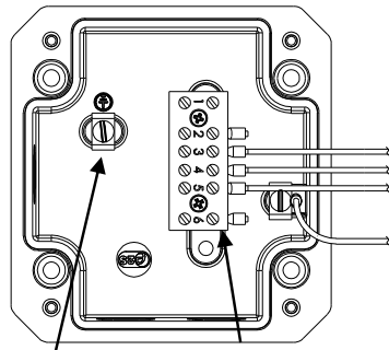
Internal Earth terminal Ex e terminal block
