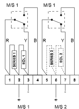
8B - Circuit shown in Operated condition (Glass Broken) Terminals +(2) & -(3) M/S 1 and +(6) & -(7) M/S 2 closed Terminals +(2) & (4) M/S 1 and +(6) & (8) M/S 2 open
