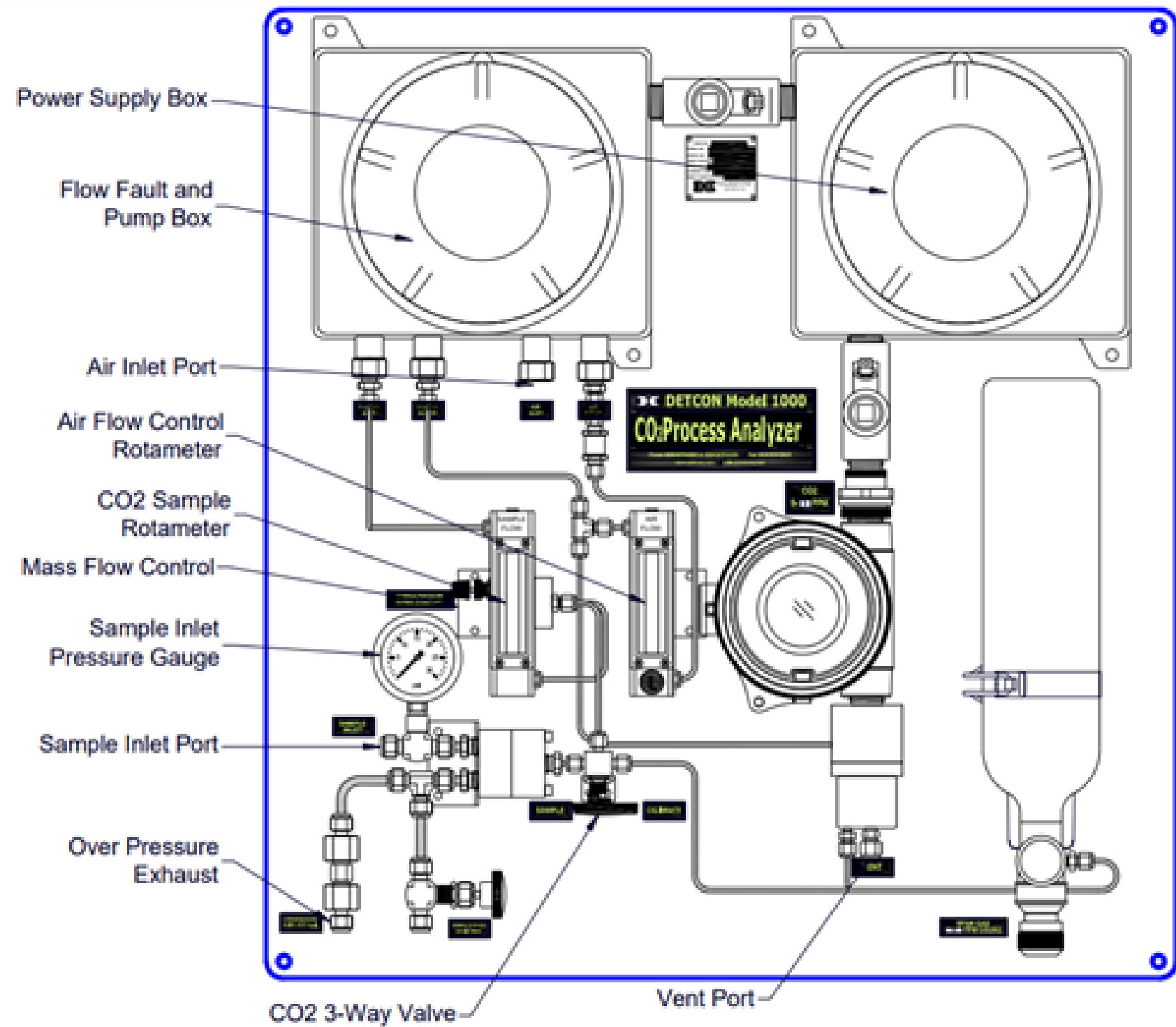
Figure 10 Unit Overview (Ir-640 0-15% with Air Dilution shown)
