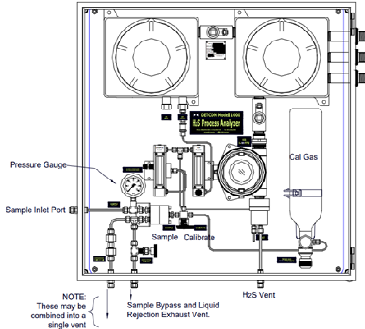
Figure 8 Port Identification
